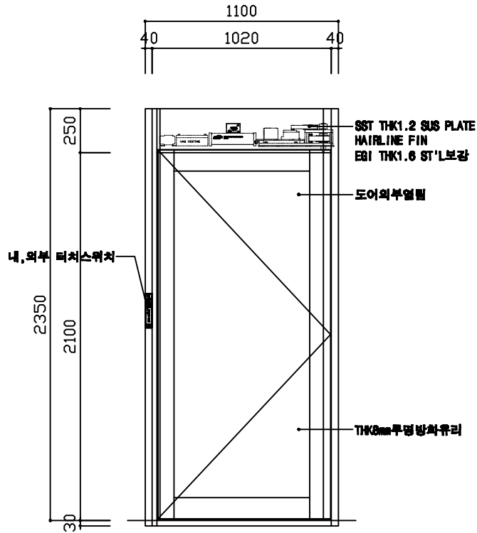
ELEVATION [EXTERIOR]
