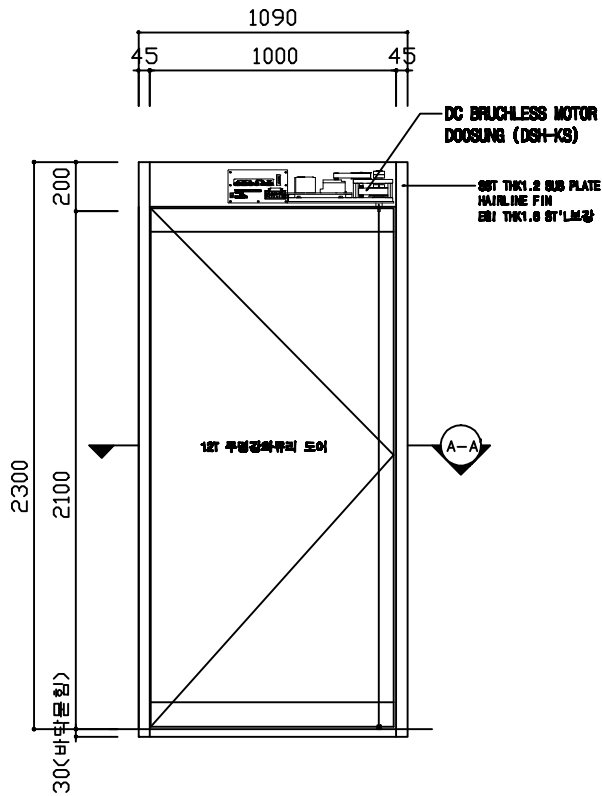
ELEVATION [EXTERIOR]
