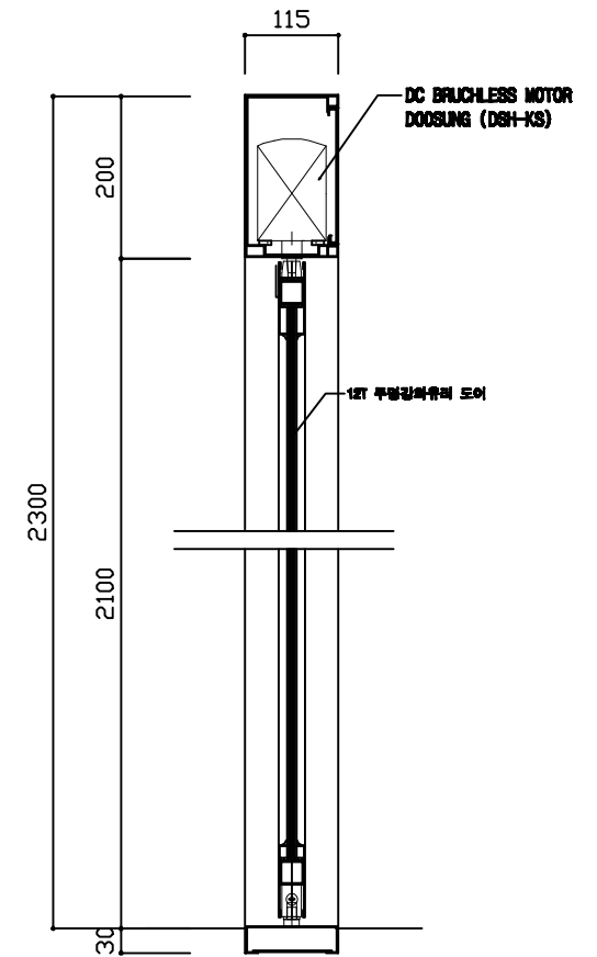
VERTICAL SECTION (OPEN)
